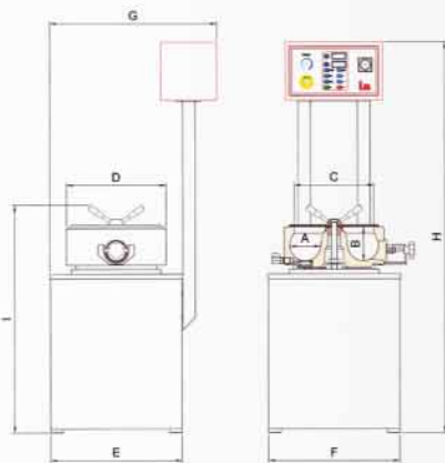
Vibratore circolare da 5-7-11-16 litri con variatore 5-7-11-16 liter circular vibrator with variable speed control
